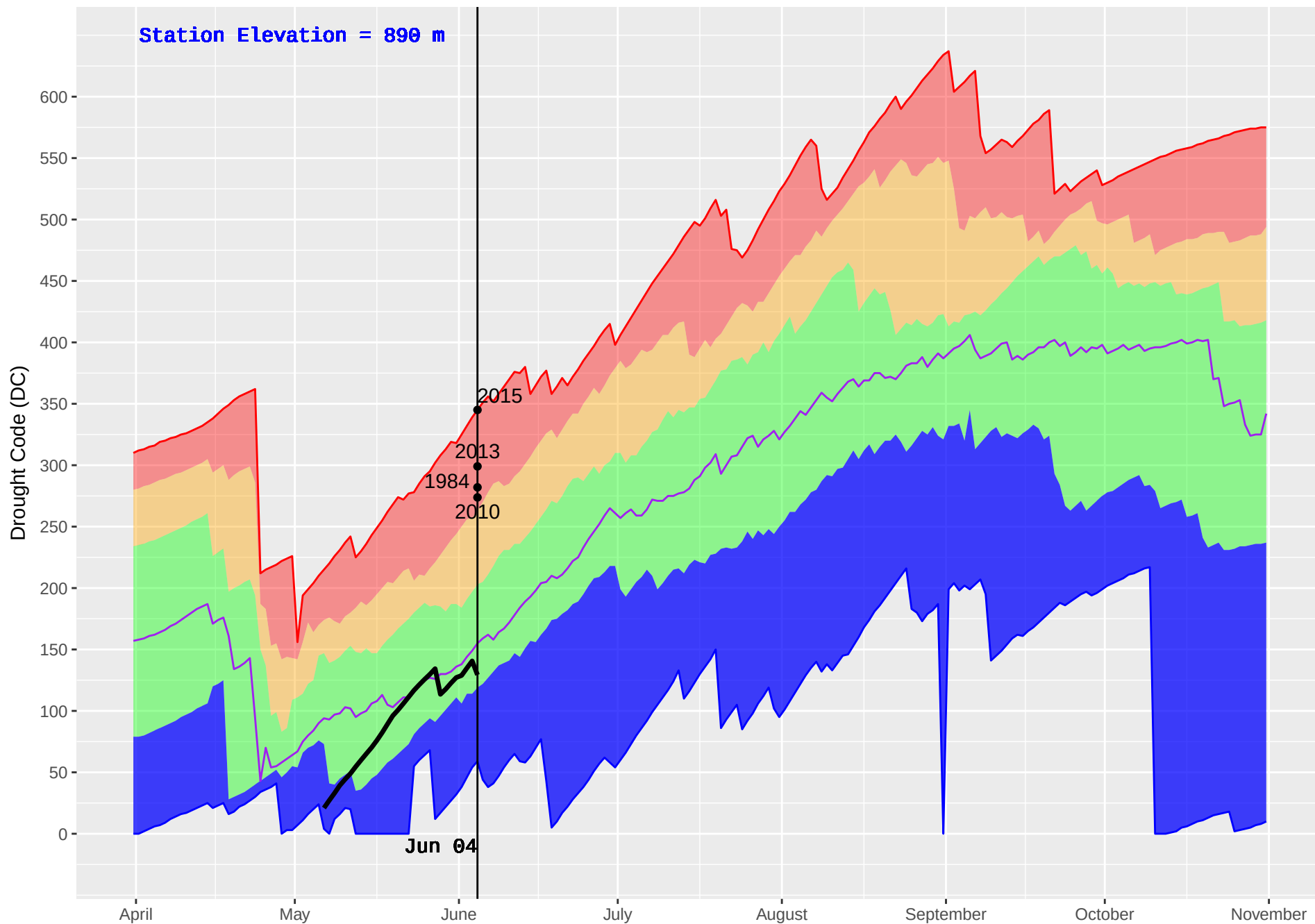
ISKUT (112) : Historical (1979–2016) and Current (2018) Noon Drought Code (DC)
